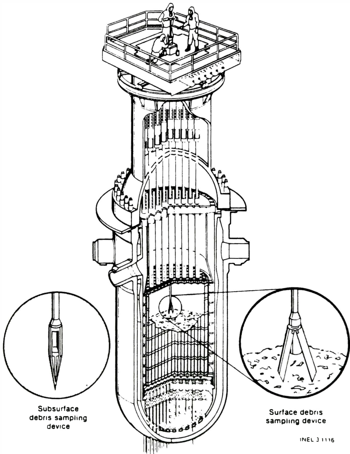
Figure 2. TMI-2 core debris sampling schematic.
