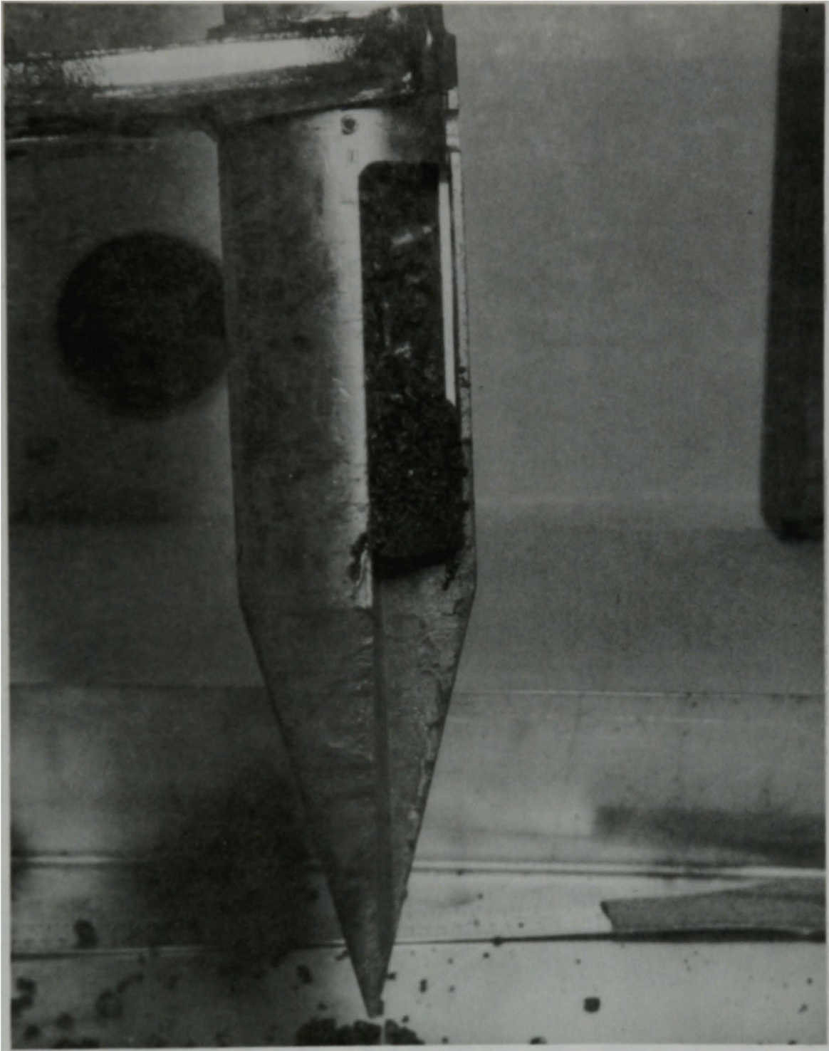
Figure 5. TMI-2 core debris sample #3 being removed from the rotating tube (22" deep-H8).
