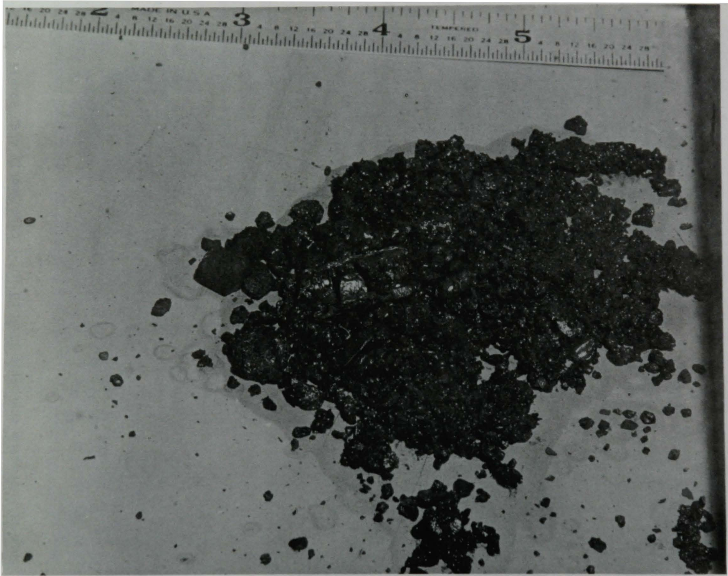
Figure 4. TMI-2 core debris sample #1 (surface-H8).
