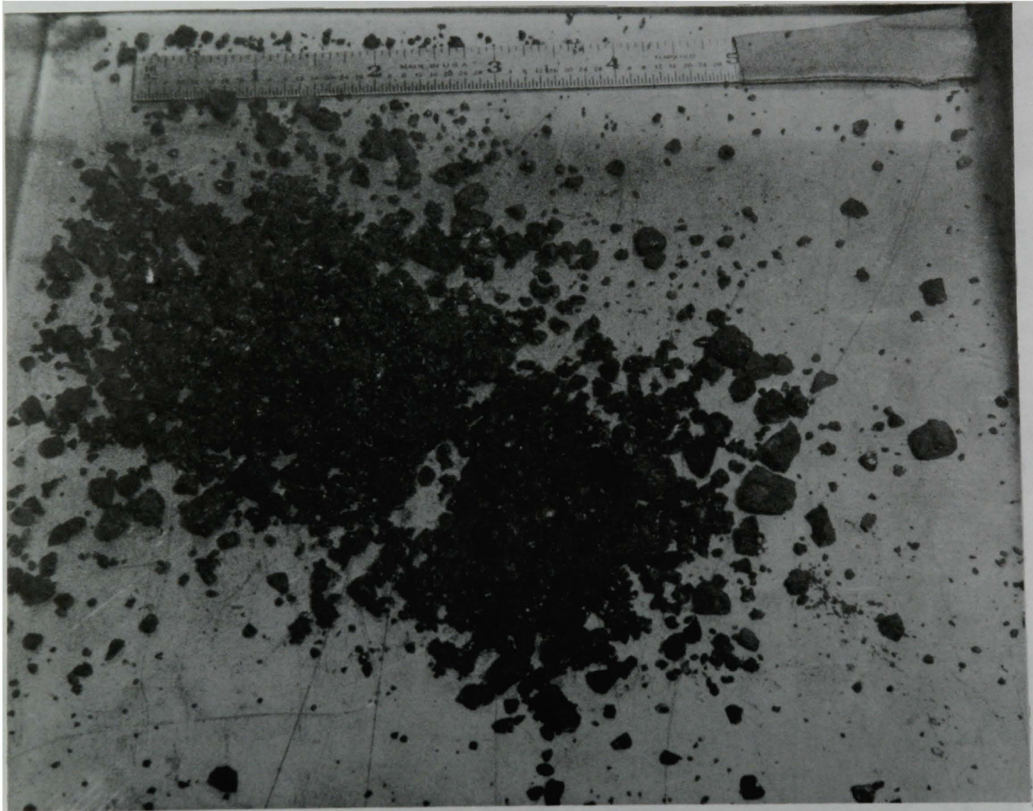
Figure 6. TMI-2 core debris sample #3 (22" deep-H8).
