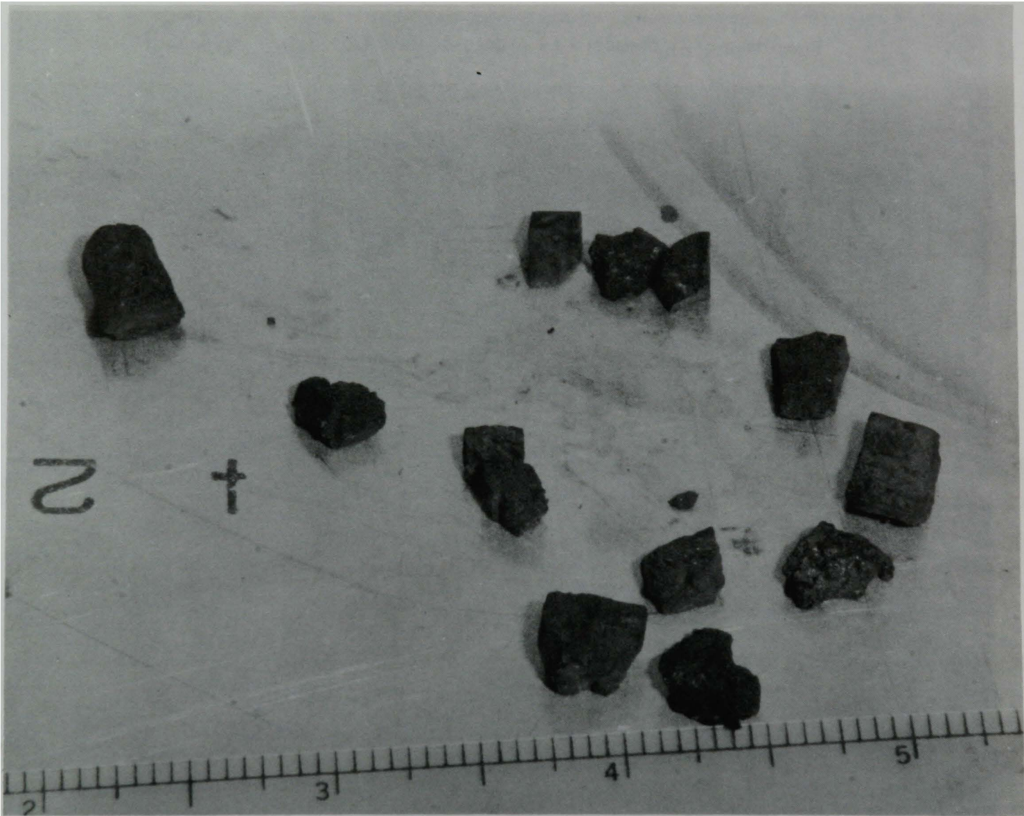
Figure 8. TMI-2 core debris sample #4 (surface-E9).
