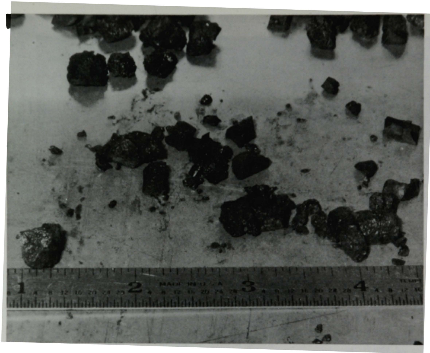
Figure 11. Close-up of TMI-2 core debris sample #5 (3" deep-E9).
