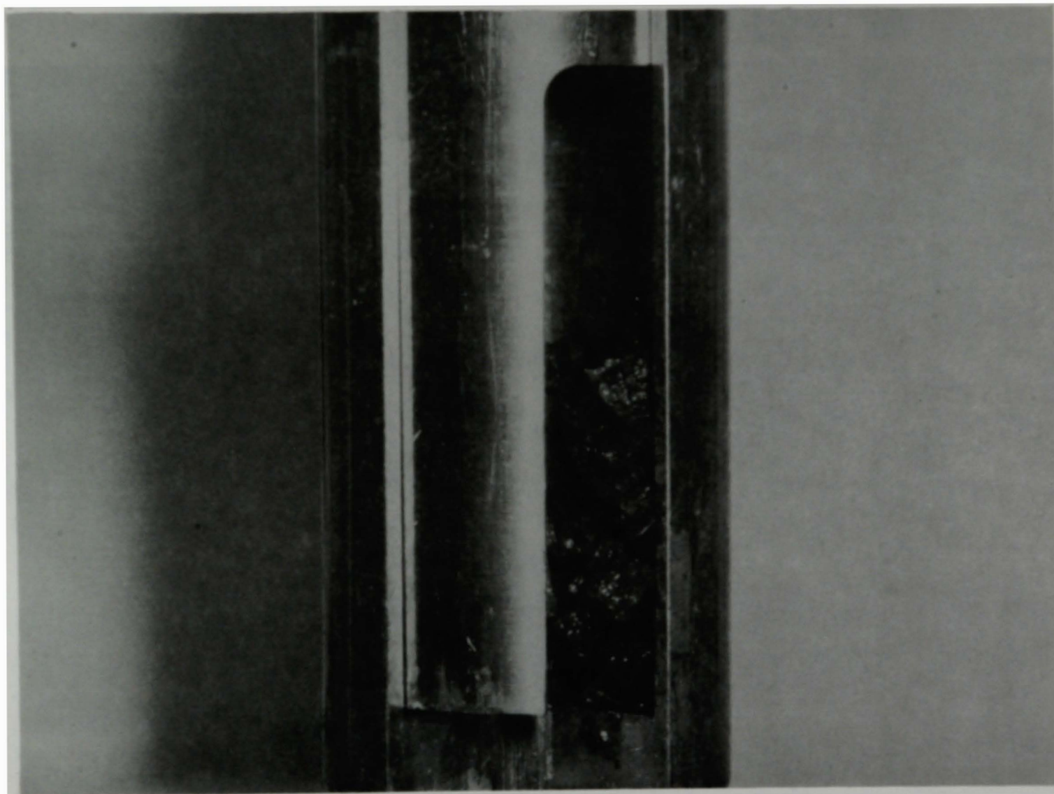
Figure 9. TMI-2 core debris sample #5 being removed from rotating tube (3" deep-E9).
