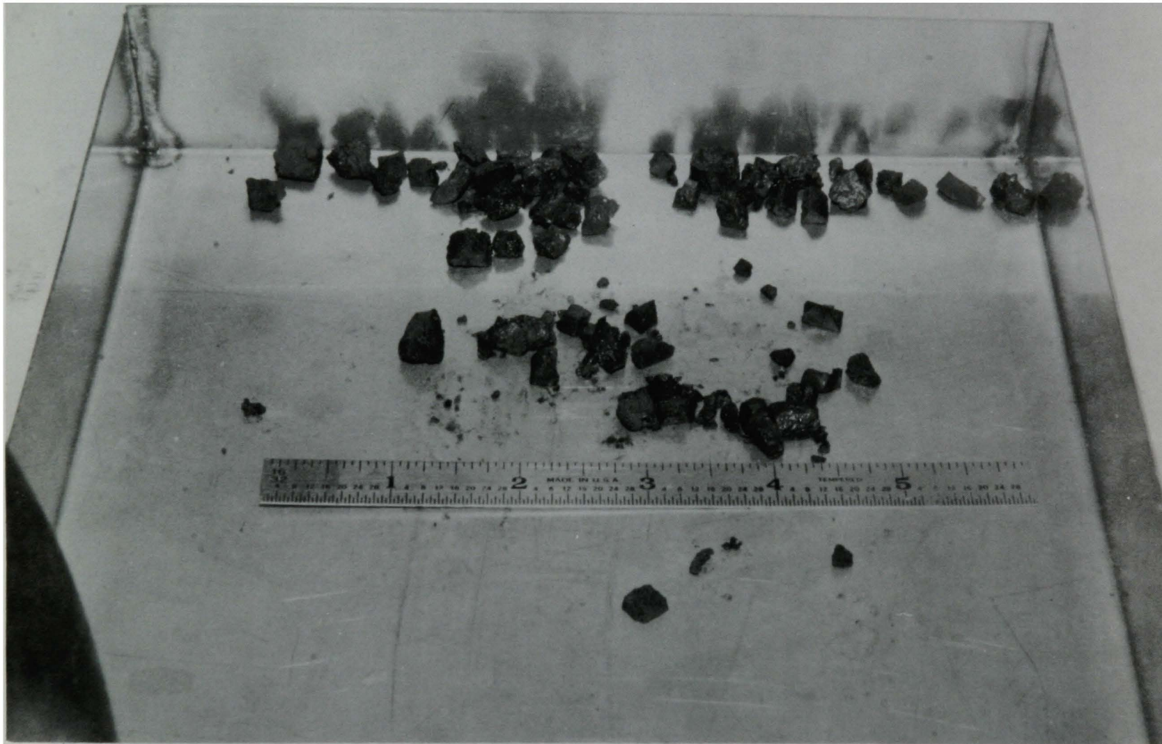
Figure 10. TMI-2 core debris sample #5 (3" deep-E9).
