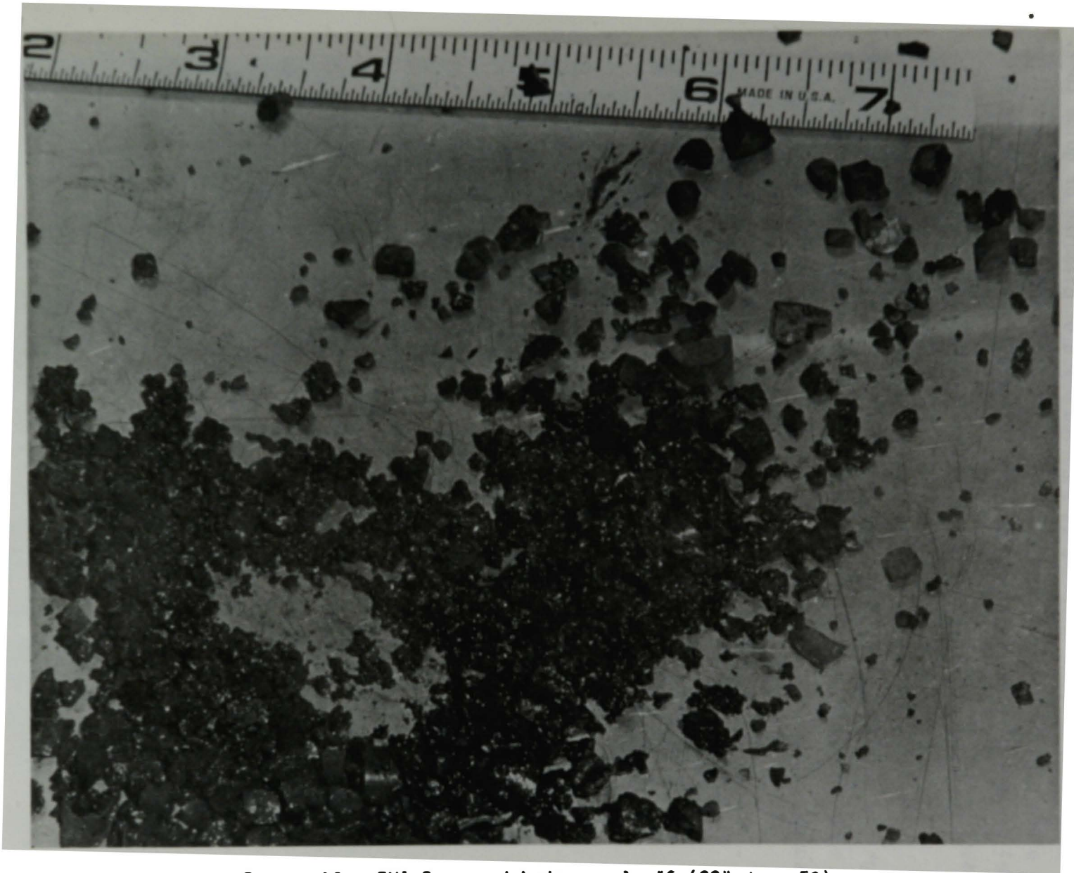
Figure 13. TMI-2 core debris sample #6 (22" deep-E9).
