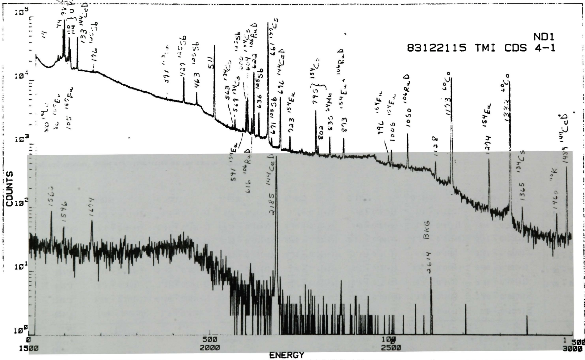
Figure 21. Gamma ray spectra for particle 4-1 removed from TMI-2 core debris sample #4 (surface-E9).
